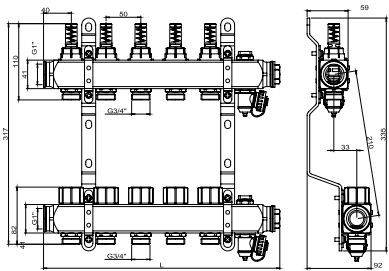
S.S. manifold with flow meters, thermostatic valves and air vents
