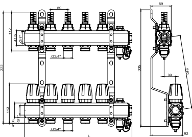
Brass manifold with flow meters, thermostatic valves and air vents
