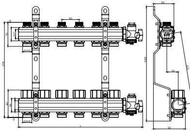
Plated brass manifold with stop valves, thermostatic valves and complex valve
