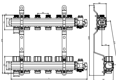
Brass manifold with stop valves, thermostatic valves and complex valve
