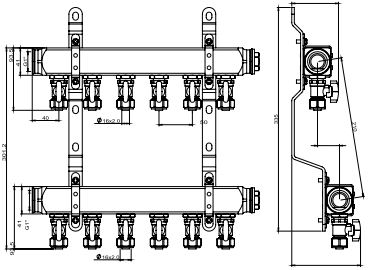
S.S. manifold G1", with connection fitting and small ball valves
