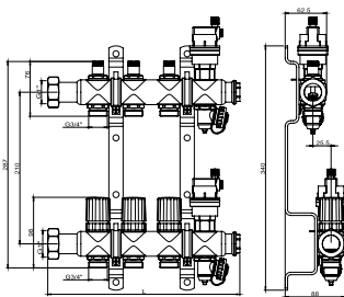
S.S. manifold with stop valves, thermostatic valves and air vents
