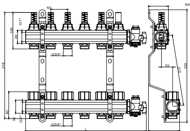
Brass manifold with flow meters, thermostatic valves and complex valve
