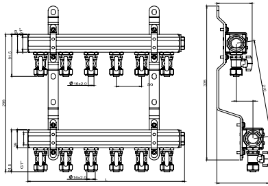
Plated brass manifold G1", with connection fitting and small ball valves
