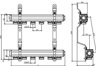
Brass manifold G1", with connection fitting
