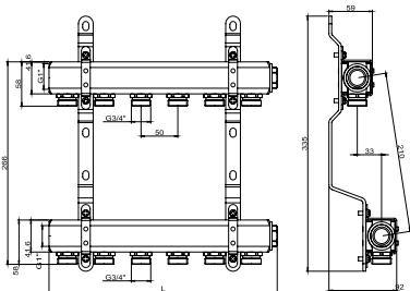
Brass manifold G1'', with connection fitting
