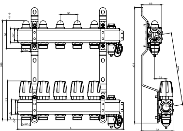
Brass manifold with stop valves, thermostatic valves and air vents
