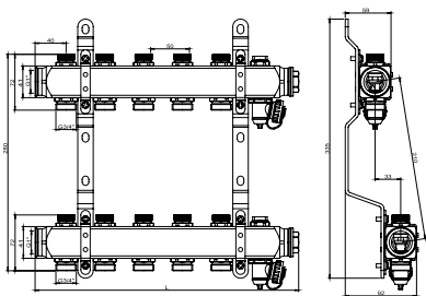
S.S. manifold with stop valves and air vents
