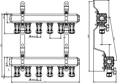
Brass manifold G1'', with connection fitting and small ball valves
