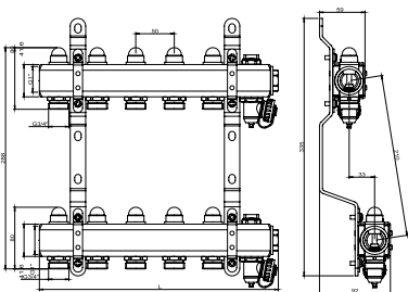
Brass manifold with stop valves and air vents
