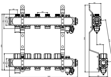
S.S. manifold with stop valves, thermostatic valves and air vents
