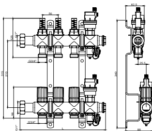
S.S. manifold with flow meters, thermostatic valves and air vents
