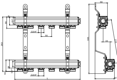
Plated brass manifold G1", with connection fitting
