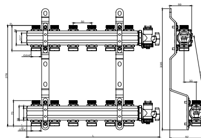
Plated brass manifold with stop valves and complex valve
