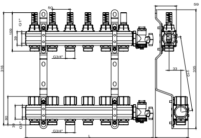
Plated brass manifold with flow meters, thermostatic valves and complex valve
