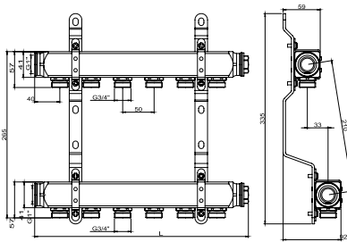
S.S. manifold G1", with connection fitting
