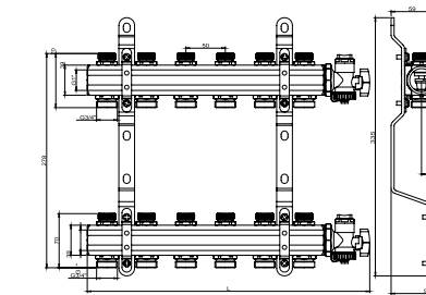
Brass manifold with stop valves and complex valve
